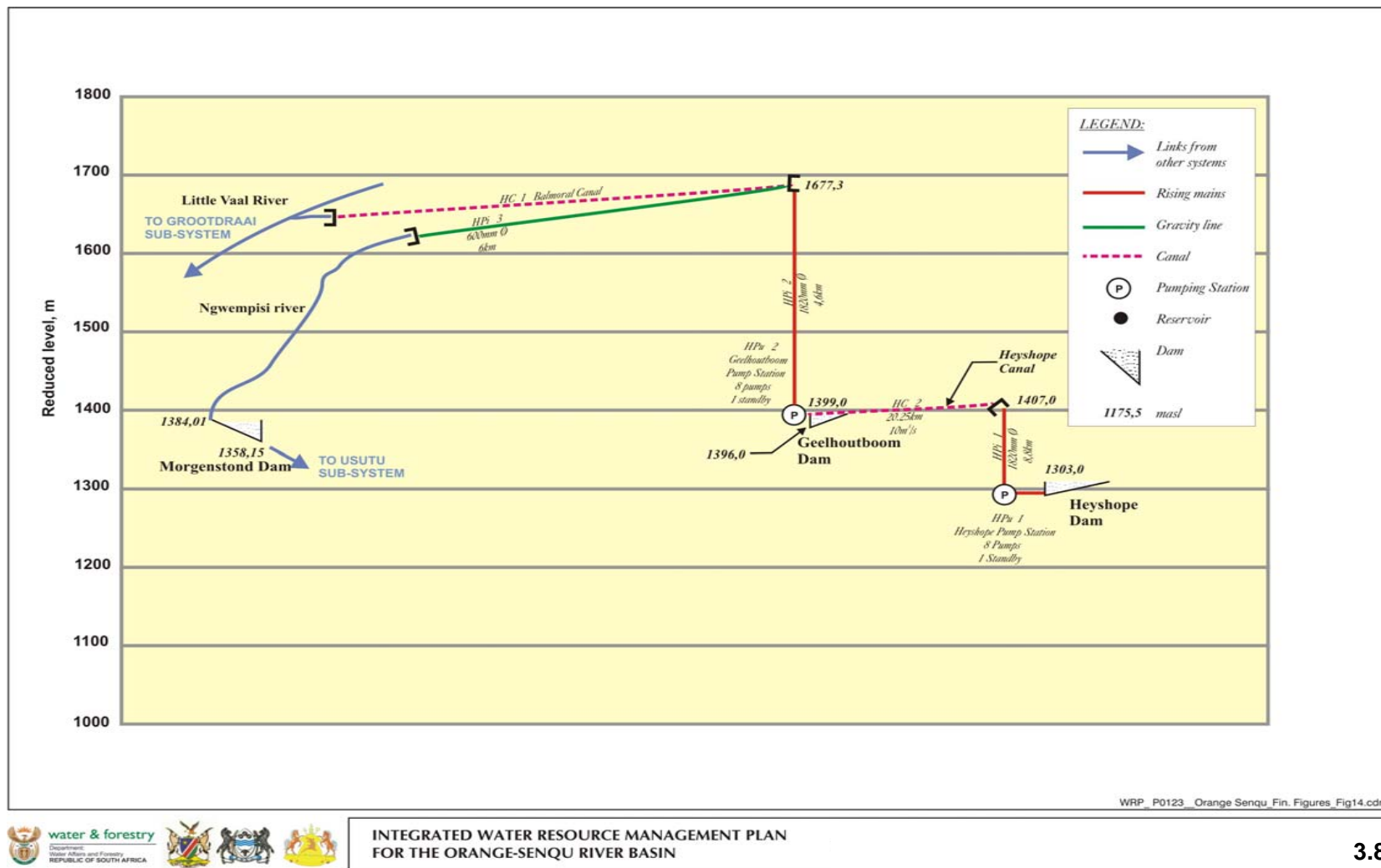
Figure 3-8: Heyshope Sam Sub-system: schematic diagram of relative elevations
