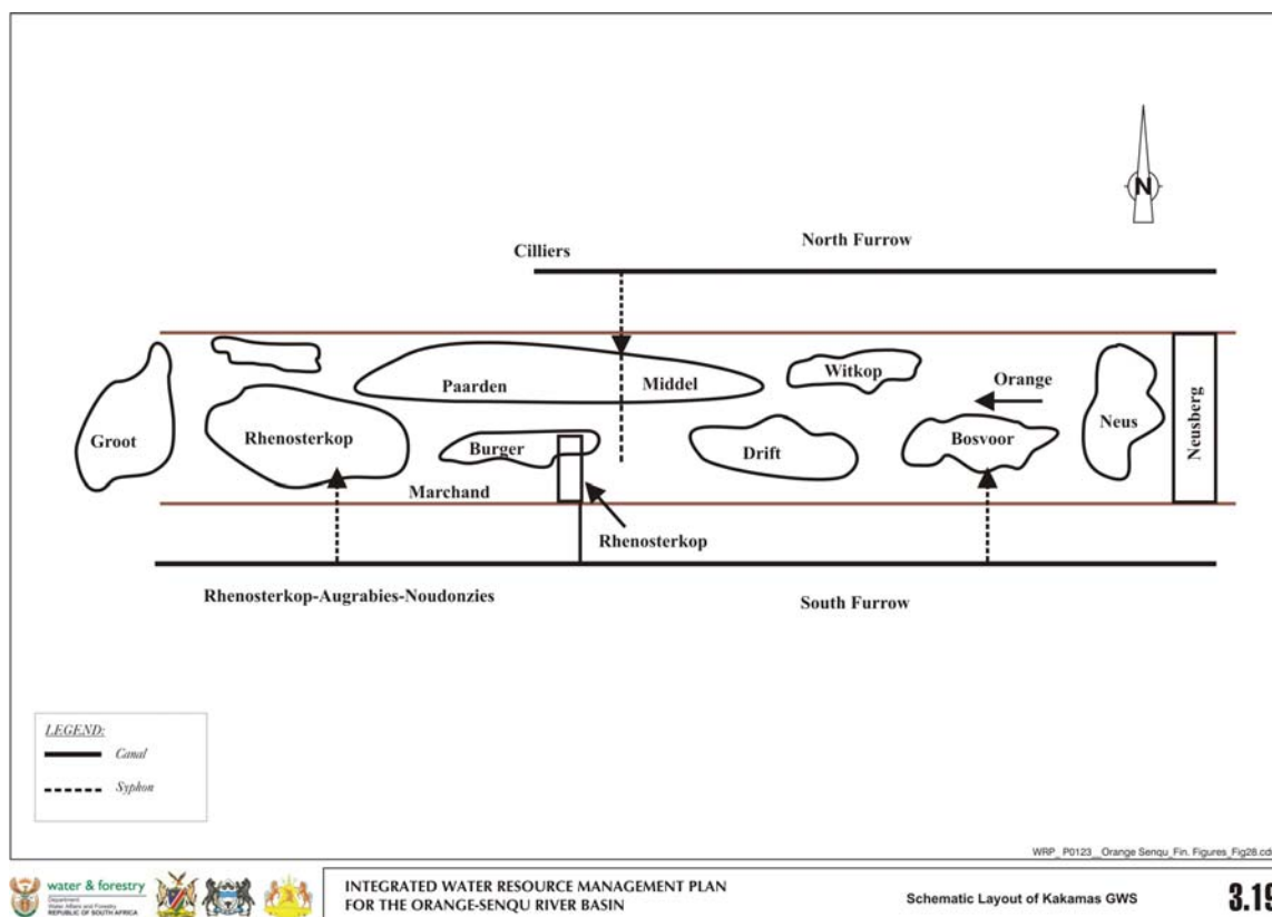
Figure 3-19 : Schematic Layout of Kakamas GWS
