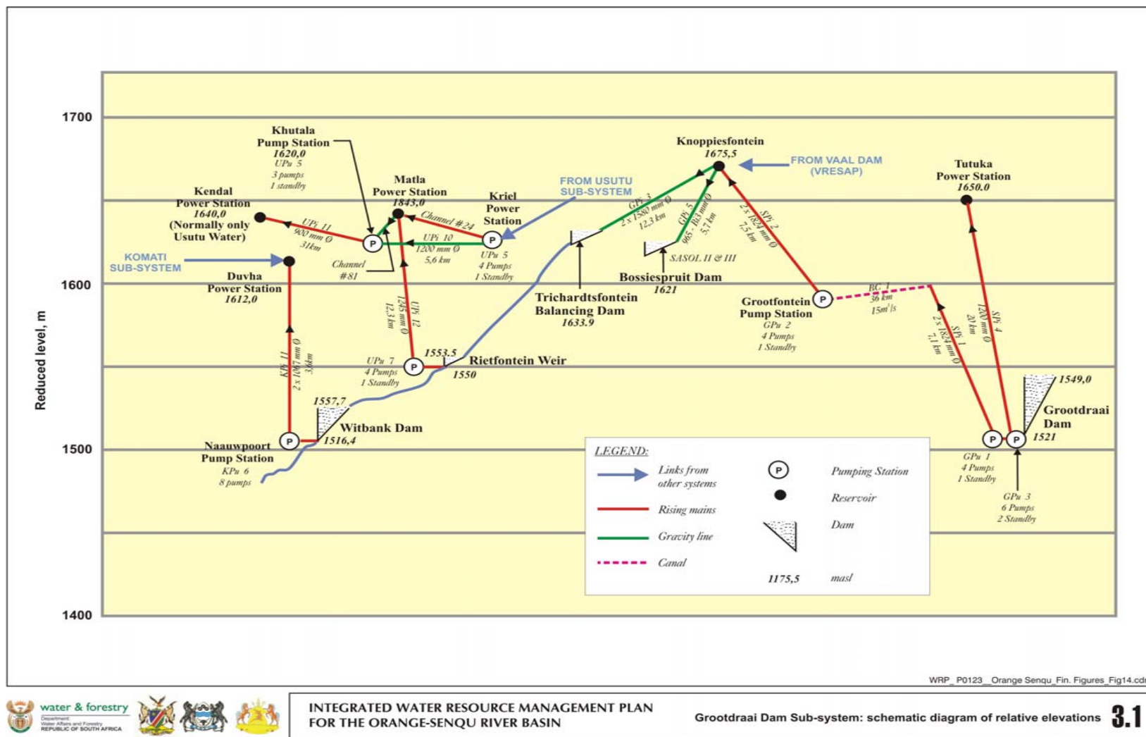
Figure 3-1: Grootdraai Dam Sub-system: schematic diagram of relative elevations
