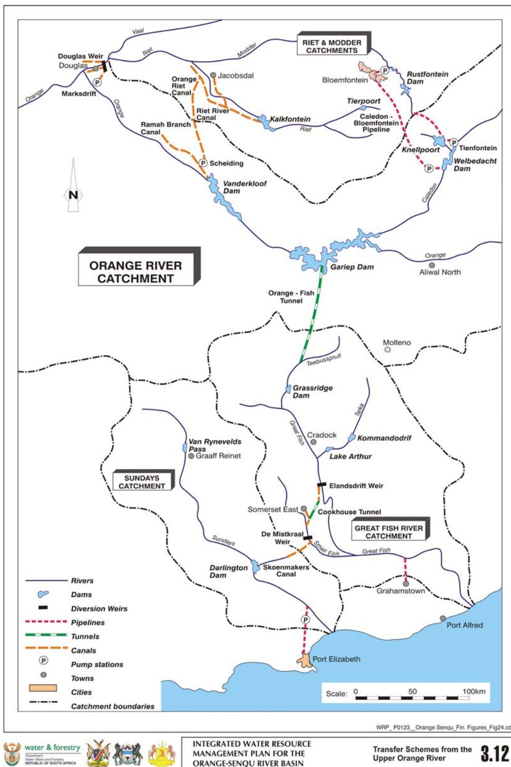
Figure 3-12: Transfer Schemes from the Upper Orange River
