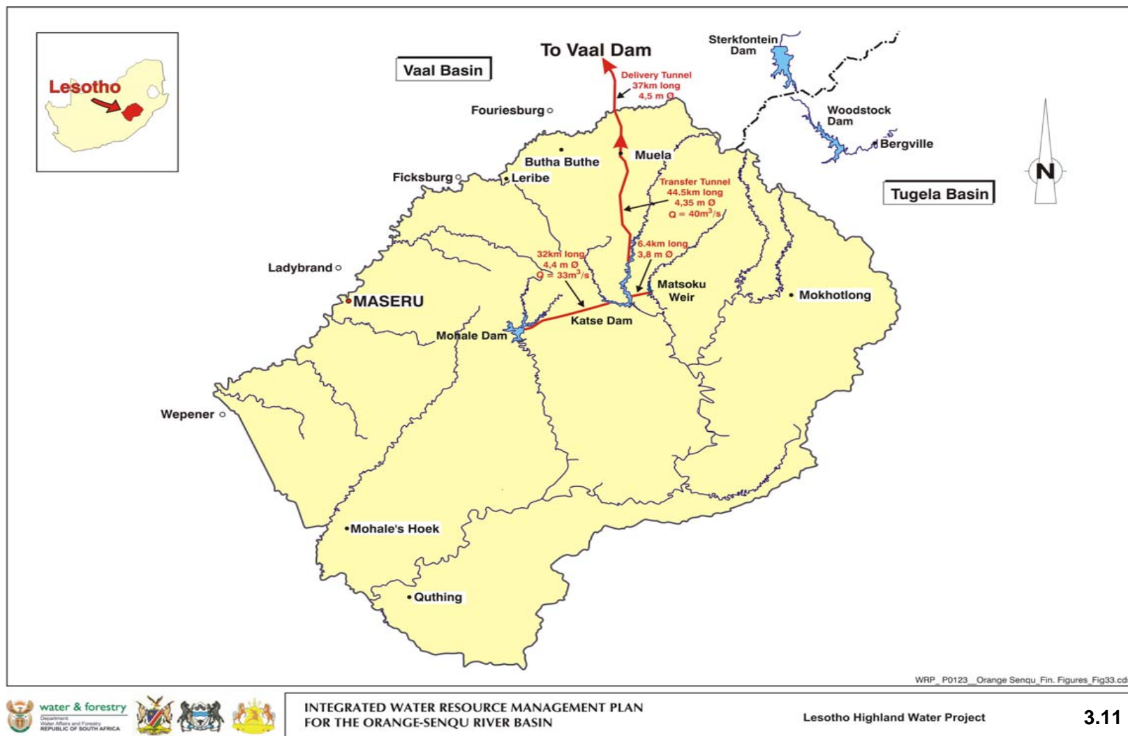
Figure 3-11: Lesotho Highland Water Project
