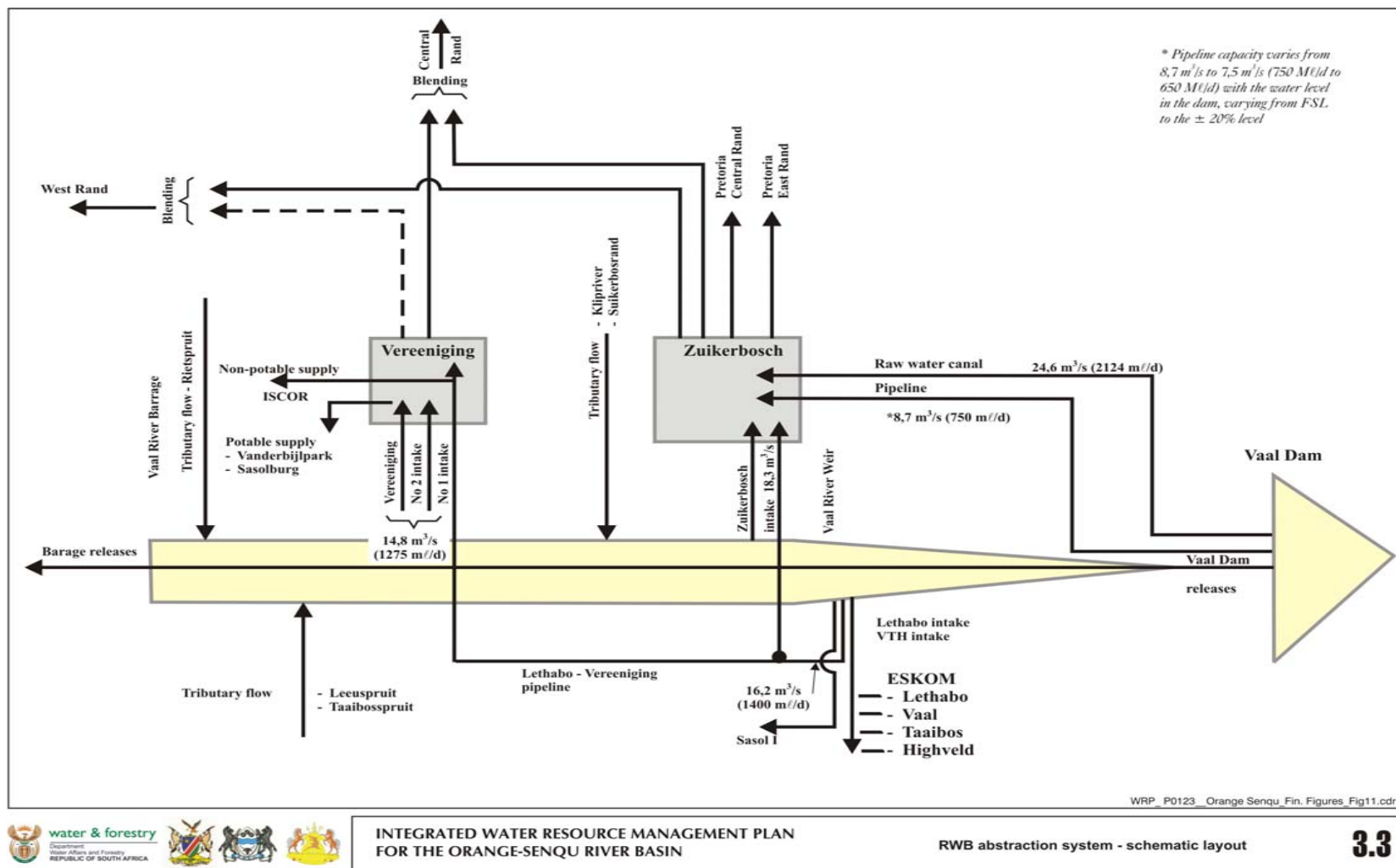
Figure 3-3: RWB abstraction system – schematic layout
