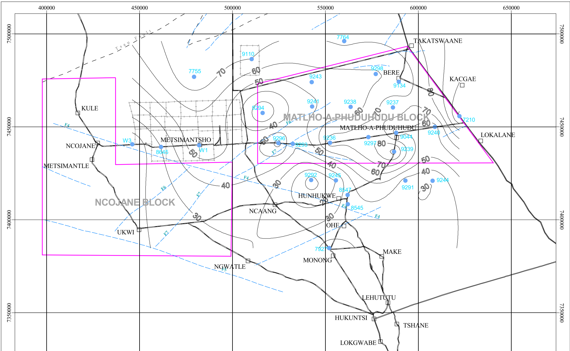
Figure 9: Thickness of the Ntane Sandstone
