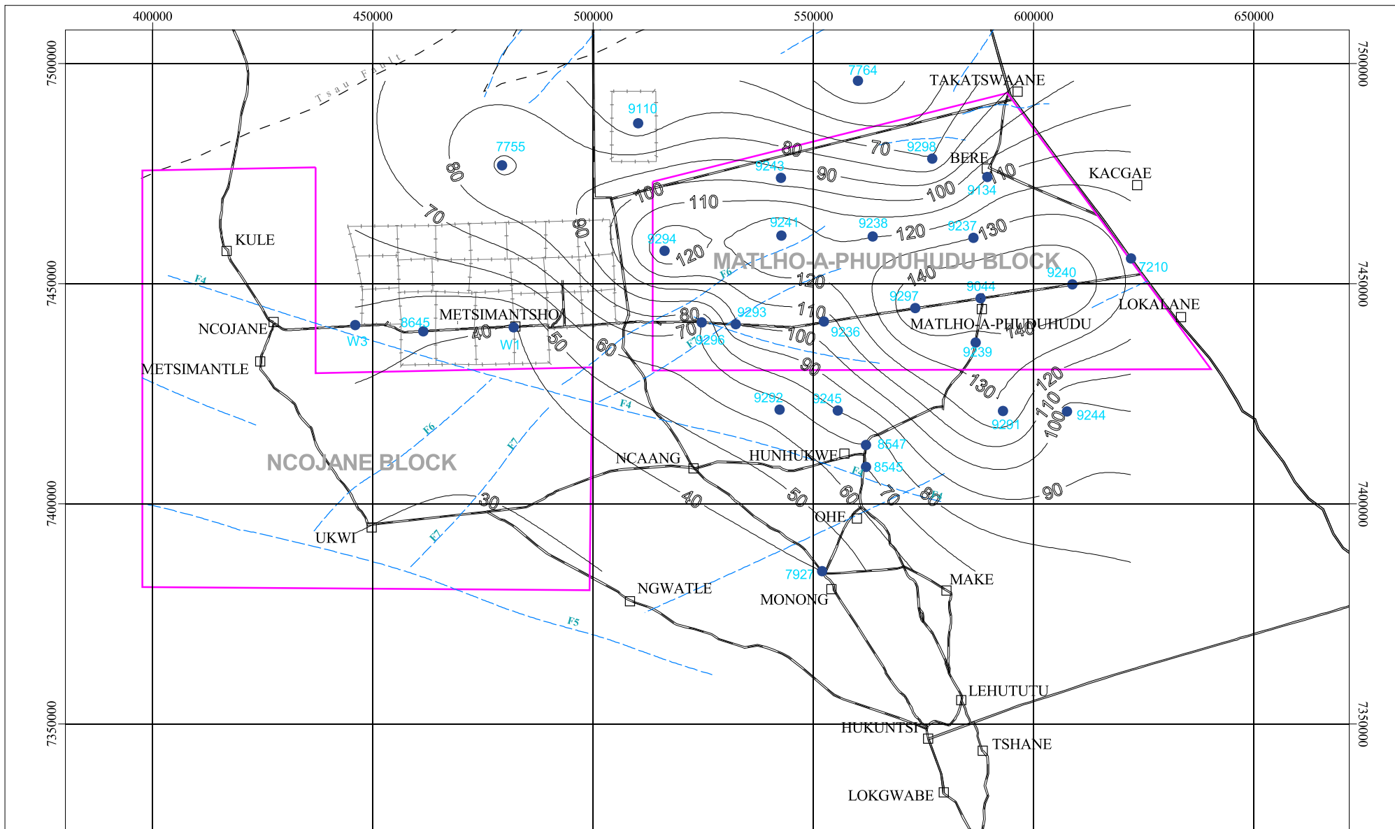
Figure 7 Depth to Top of the Ntane Sandstone
