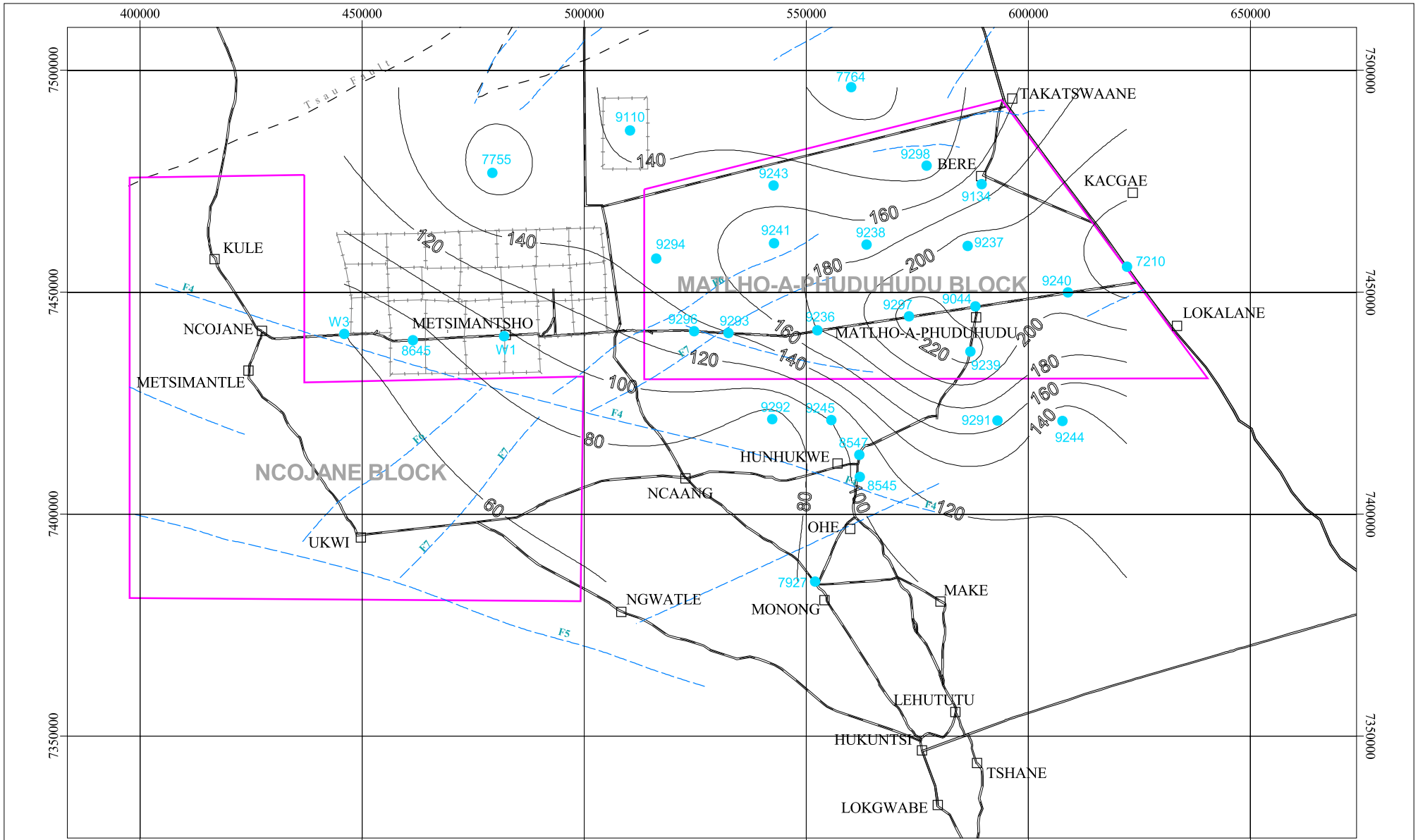
Figure 8 Depth To Bottom of the Ntane Sandstone
