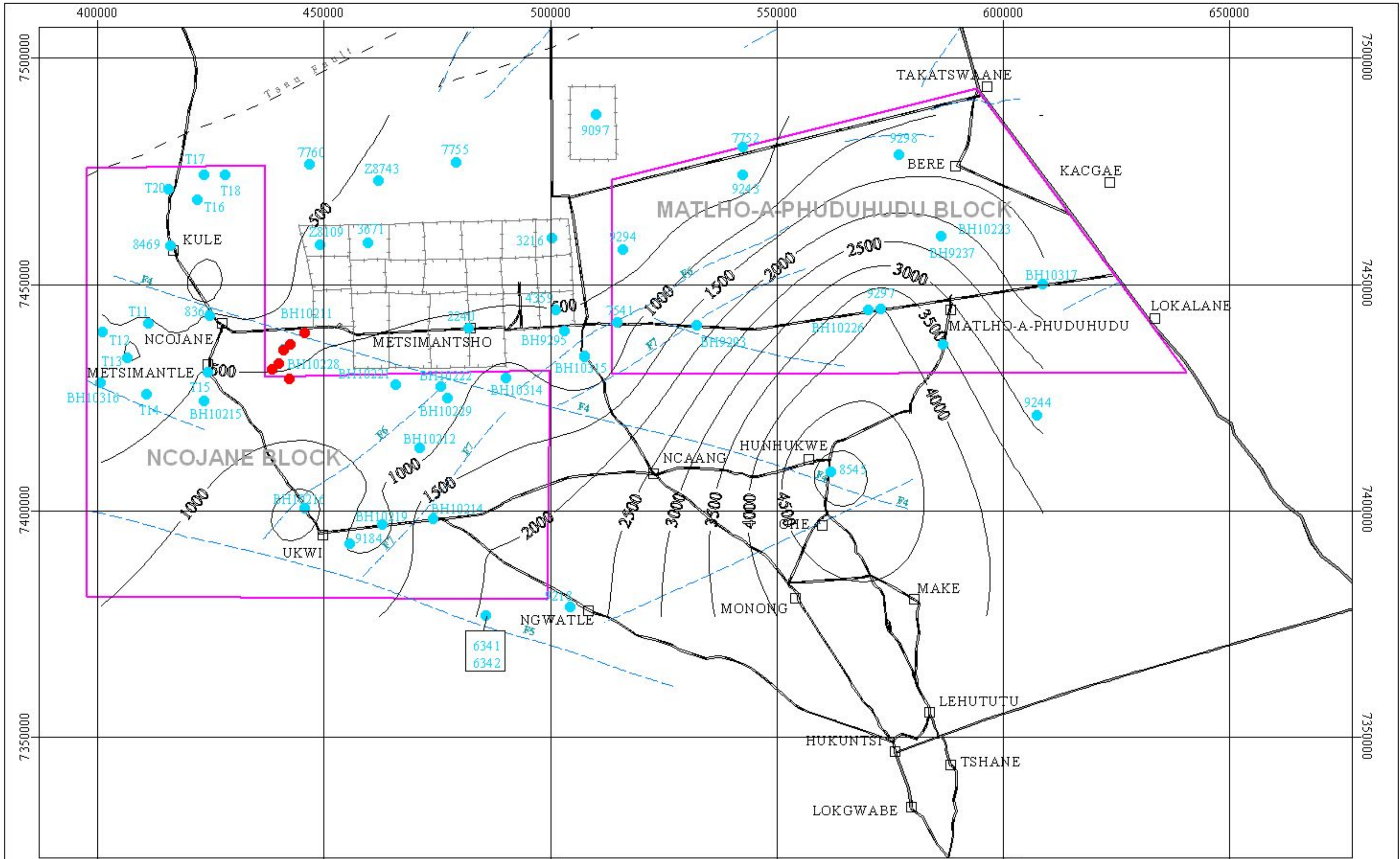
Figure 18: TDS Distribution Ecqa (Otshe) Aquifer
