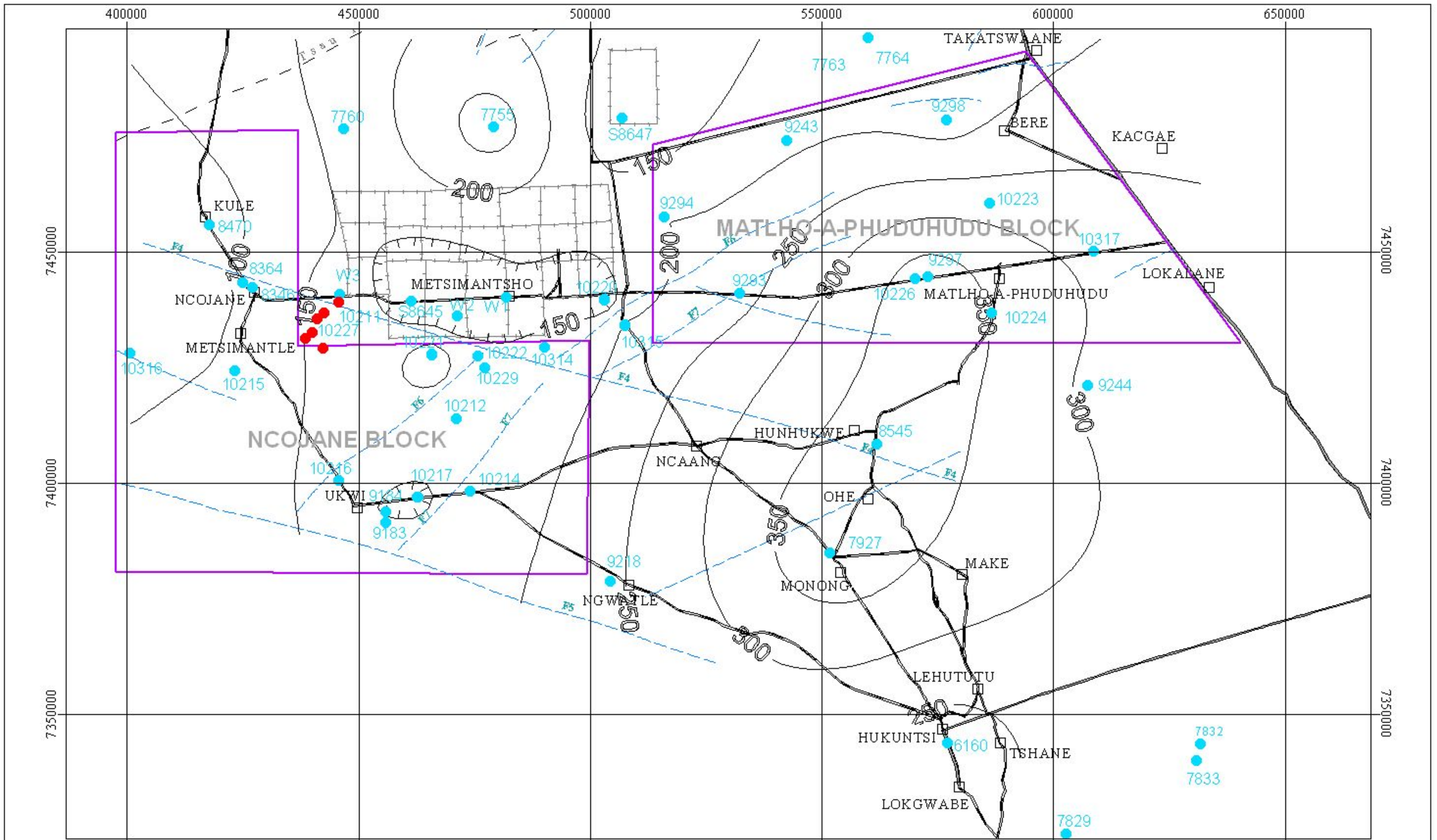
Figure 16: Depth to Top of Ecca Group
