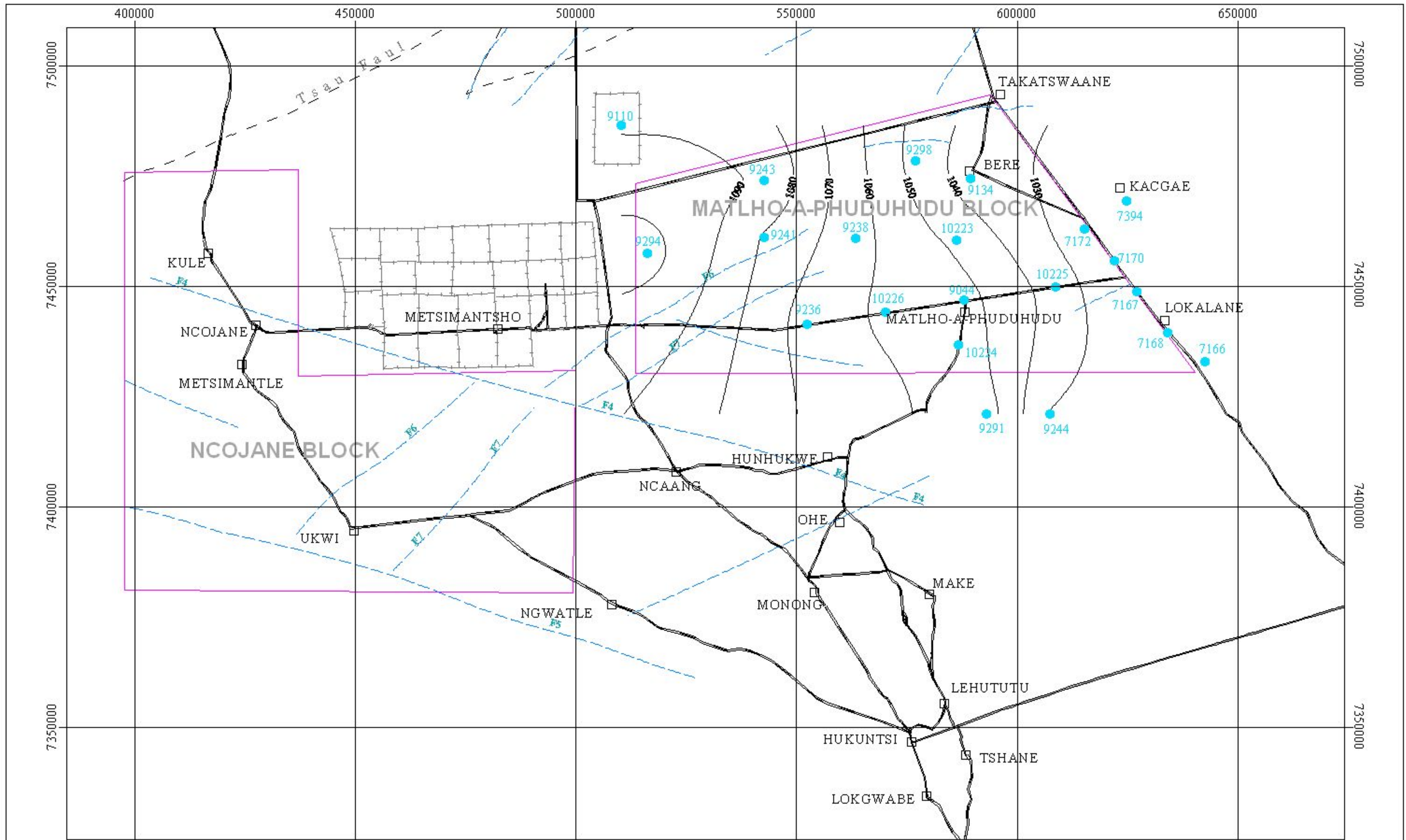
Figure 12: Piezometric Head Ntane Sandstone
